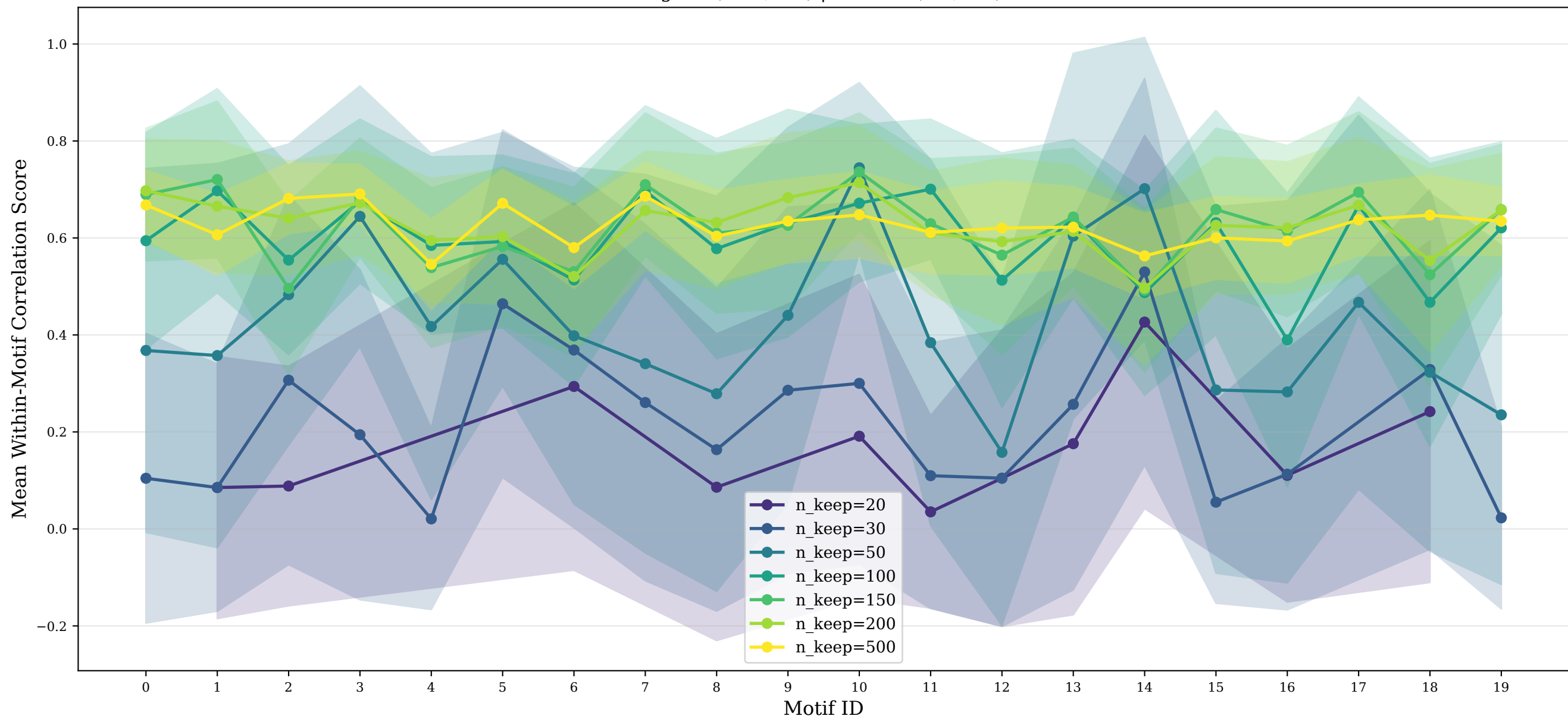
Correlation Score per Motif at Different Downsampling Levels (min_length=5) sigma: (0.02, 0.4) | volume: (0.1, 0.5)
